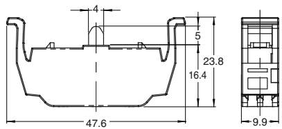
Contact Blocks (Single Contact) A22NZ-S-P1□
